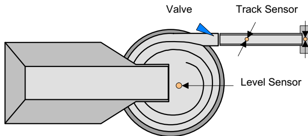
Hopper Feeder
